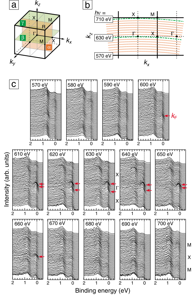
FIG. 1. (Color online) (a) The schematic of a cubic Brillouin zone. (b) The momentum space region of the ARPES measurements. (c) The EDCs at photon energies between h\nu=570 and 700 eV at normal emission.
