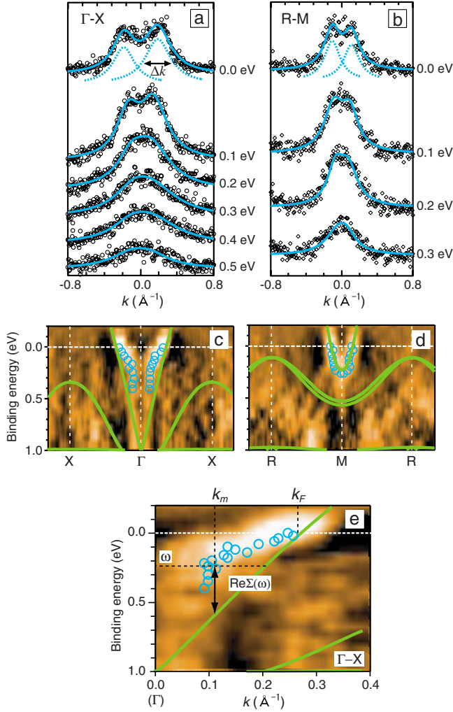
FIG. 4. (Color online) (a) and (b) MDCs with fitted spectra using two Lorentzians. (c) and (d) The intensity map of the second derivative MDCs with LDA band calculation [green (gray) lines]. The experimental band dispersion derived from the peak positions of second derivative MDCs is shown as the blue (gray) circles. (a) and (c) were measured along \Gamma - X direction, while (b) and (d) were measured along R - M direction. (e) Expanded view of the intensity map of the second derivative MDCs with LDA band calculation [green (gray) lines] in \Gamma - X direction.
