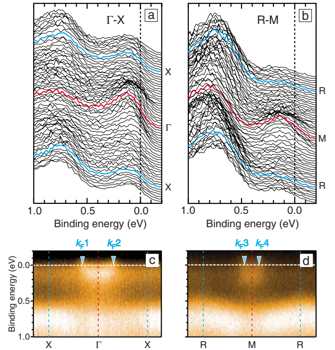
FIG. 3. (Color online) (a) and (b) EDCs along \Gamma - X and R - M direction, respectively. (c) and (d) The intensity maps of EDCs. k_{F1} - k_{F4} indicate the MDC peak positions at E_F .
