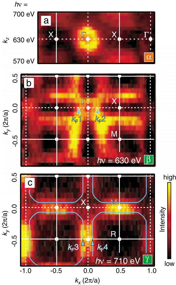
FIG. 2. (Color online) Fermi-surface mapping in (a) a vertical ( k_z - k_x ) plane “ \alpha ” and (b) horizontal ( k_x - k_y ) planes “ \beta ” and (c) “ \gamma ” of Brillouin zone in Fig. 1(a). Solid white lines correspond to the cubic Brillouin zone and dotted white lines correspond to the high-symmetry lines. k_{F1} - k_{F4} indicate the MDC peak positions at E_F in Figs. 3(c) and 3(d). Blue (gray) lines show nesting character hole FSs. All the intensity maps are measured data over the displayed range and no symmetrization has been used to obtain the maps.
